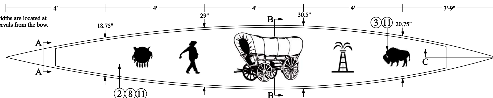
Plan View Scale: 1" = 2'
